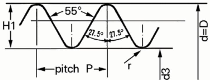
FIGURE 13 Devised by Sir Joseph Whitworth in 1841, this standardised screw has a thread angle of 55° and a depth of 0.640327p and a radius of 0.137329p, where p is the pitch. The need for mass production of weaponry during the Crimean War gave impetus to the adoption of the Whitworth standard, and it is still widely in plumbing fixtures and in some computer applications in the United States.
